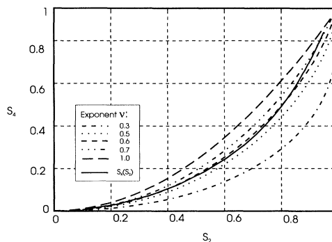
FIG. 10. Functional dependence of S_4 on S_2 according to the principle of maximum entropy together with various fit functions.
