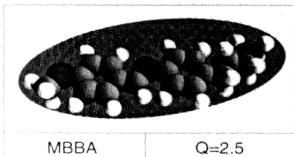
FIG. 4. Space filling model of MBBA and enclosing ellipsoid with axis ratio 2.5.
