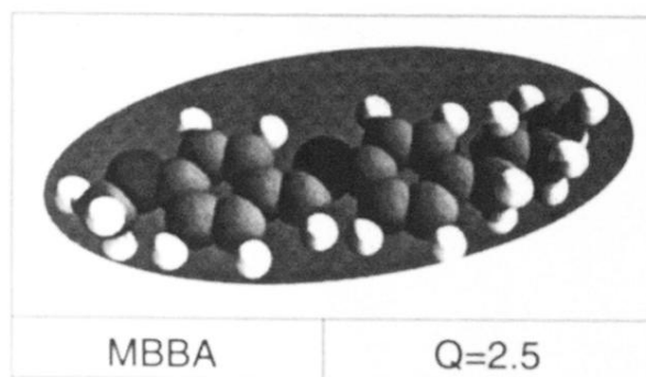
FIG. 4. Space filling model of MBBA and enclosing ellipsoid with axis ratio 2.5.
