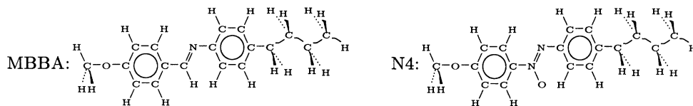
FIG. 3. Structural formulas of MBBA and N4 (isomeric mixture).
