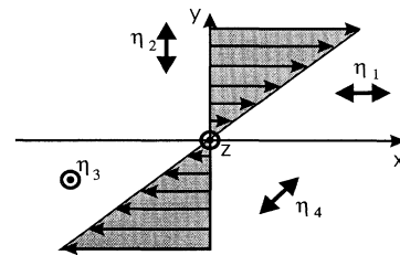
FIG. 1. Geometry of a plane Couette flow and definition of the Miesowicz viscosities.
