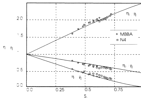
FIG. 5. Miesowicz viscosities of MBBA and N4 (data from [29,28] using Haller's equation [21]).
