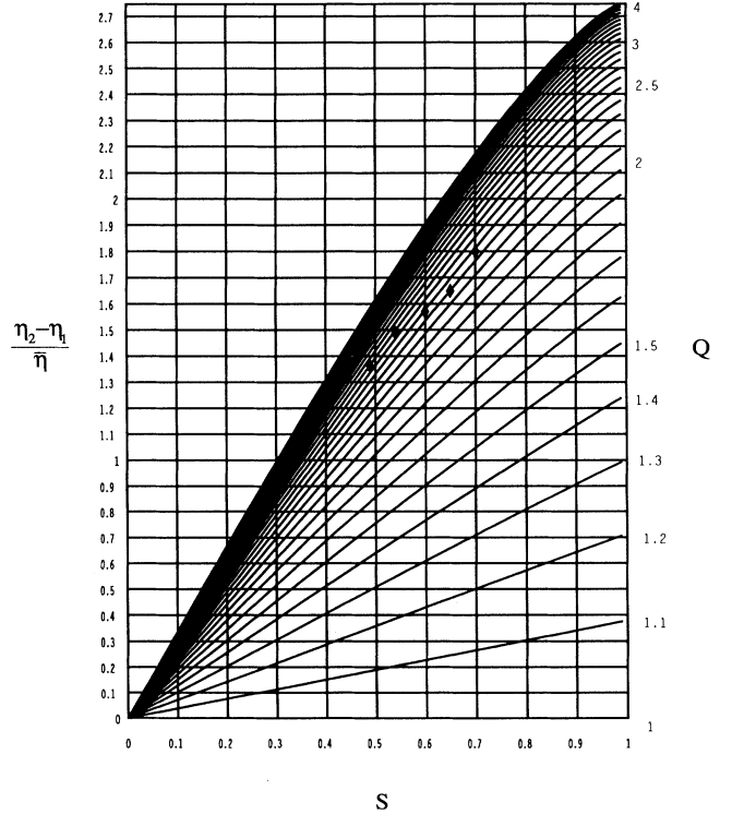
FIG. 2. Determination of the axis ratio Q of N4 (experimental values (taken from [28]) are marked with a filled \diamond ).
