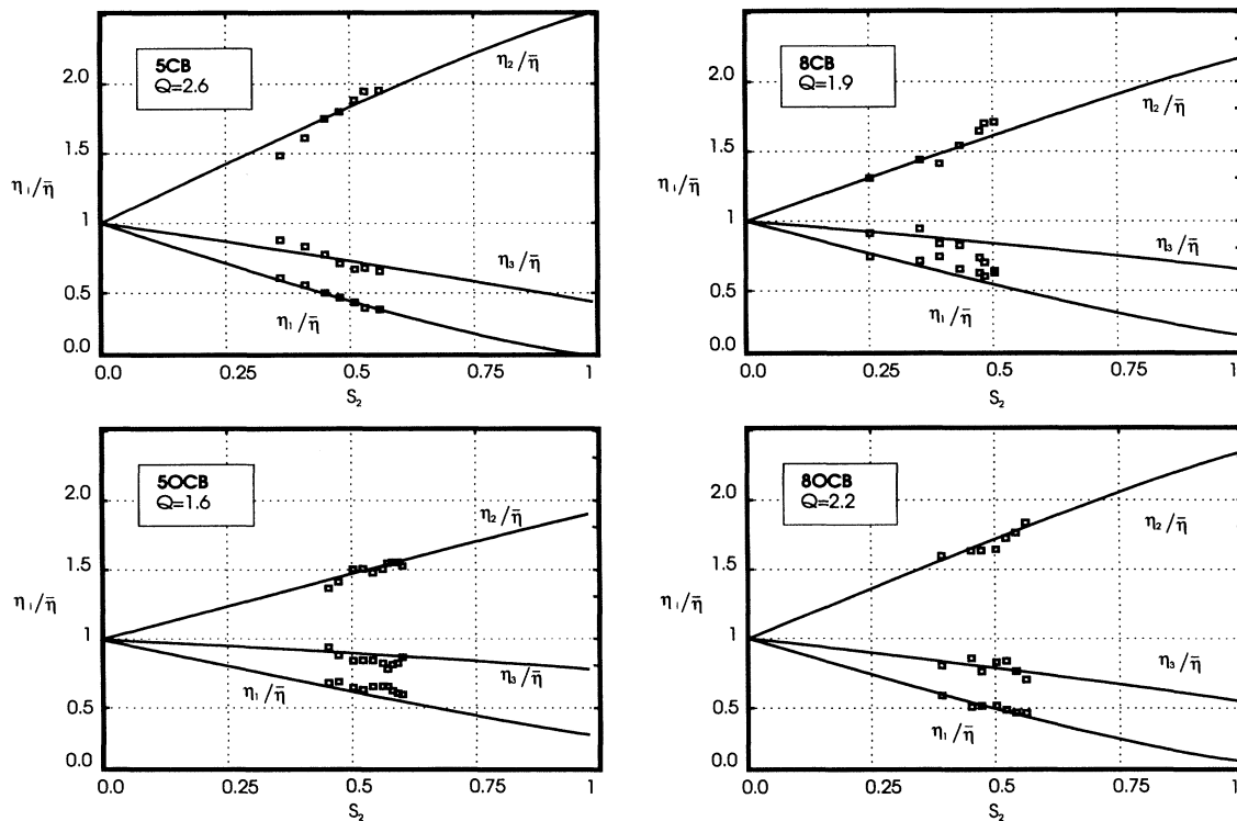
FIG. 8. Relative Miesowicz viscosities of k CB and k OCB ( k = 5, 8 ); data taken from [22].
