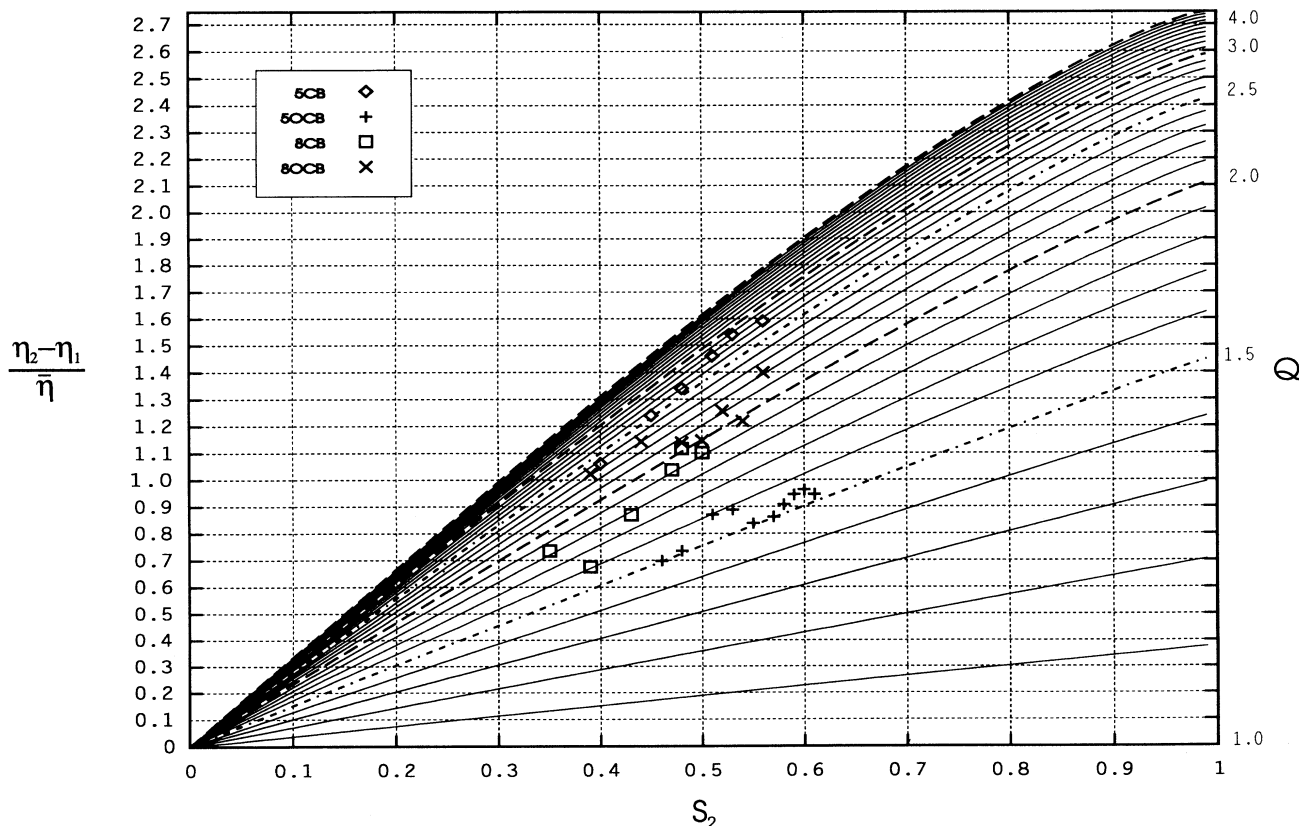
FIG. 7. Determination of axis ratios of k CB and k OCB ( k = 5, 8 ).
