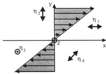
FIG. 1. Geometry of a plane Couette flow and definition of the Miesowicz viscosities.
