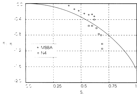
FIG. 6. Comparison of \eta_{12} with experimental values [29,28]. The order parameter S_2 is derived from temperature by the help of Haller's equation [21].
